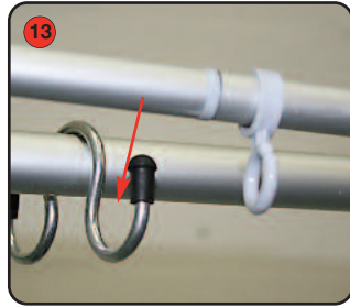
13 Rest the top bungee pole (pole WITHOUT metal rings) onto each support hook.
