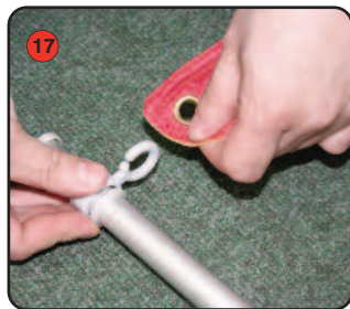
17 Take the bottom horizontal edge of the graphic and attach each eyelet onto the plastic hooks on the bottom bungee pole. Space out evenly. For double sided display repeat steps 14 to 17 for the 2nd graphic
