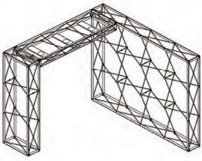
LED Kit for Bridge 9 Watt
