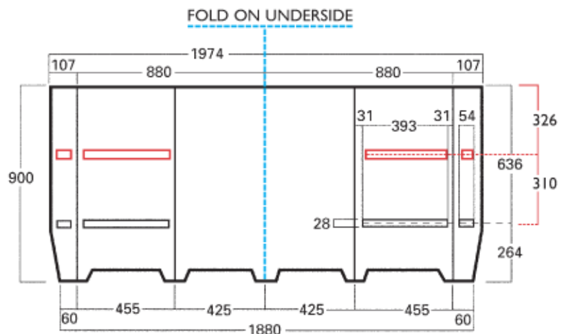
GRAPHIC SIZE FOR ONE AND TWO SHELF UNIT
